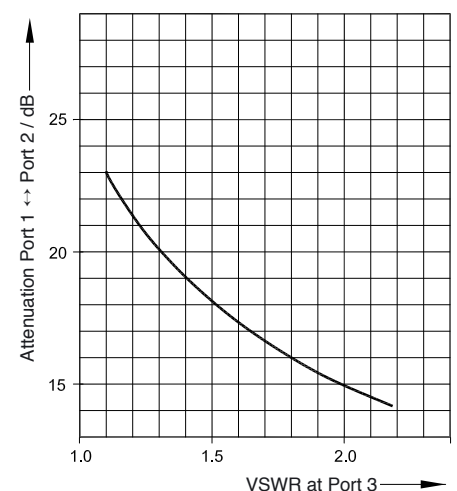
Typical attenuation Port 1 ↔ Port 2 vs. VSWR at Port 3
