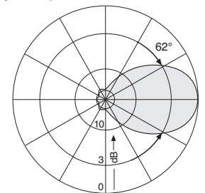
in H-plane Vertical Radiation Pattern
